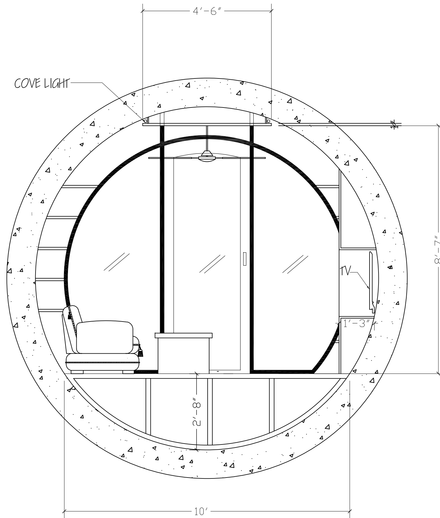
SECTION: BB'
